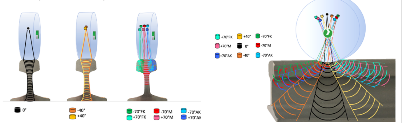
SoniQ Rail Explorer test wheel concept
